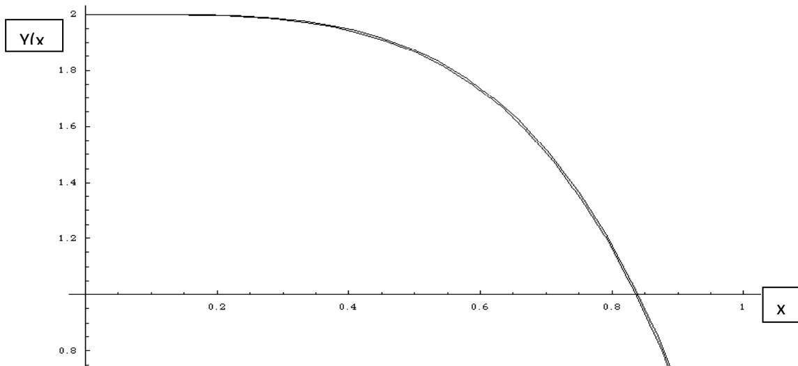
Figure 1: Comparison for \epsilon = 0.0002 and \mu = 0.001 with small values of x
