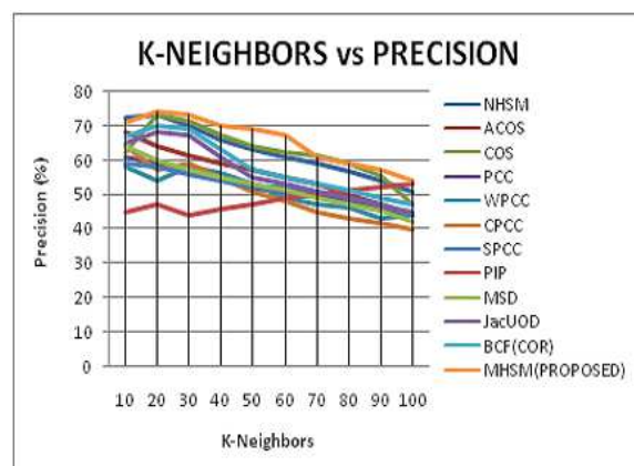
Fig. 7: Comparison of precision against K-Neighbors on News data set.
