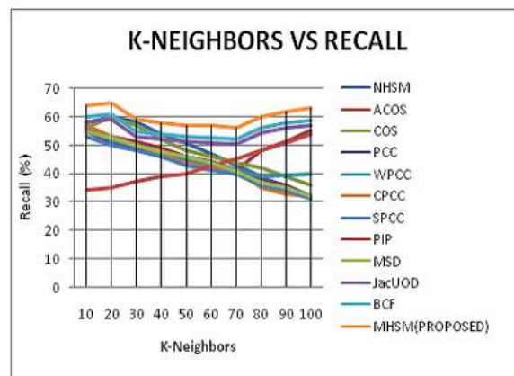
Fig. 8: Comparison of Recall against K-Neighbors on News data set.
