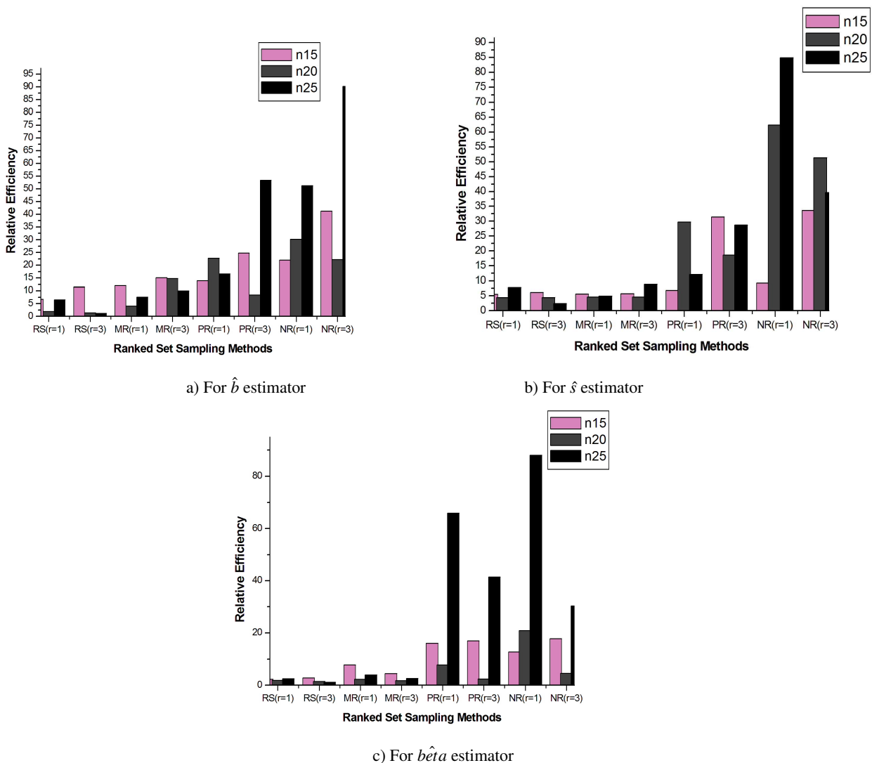
Fig. 1: shows the REs of the estimators for G/G(2,2,4) .
