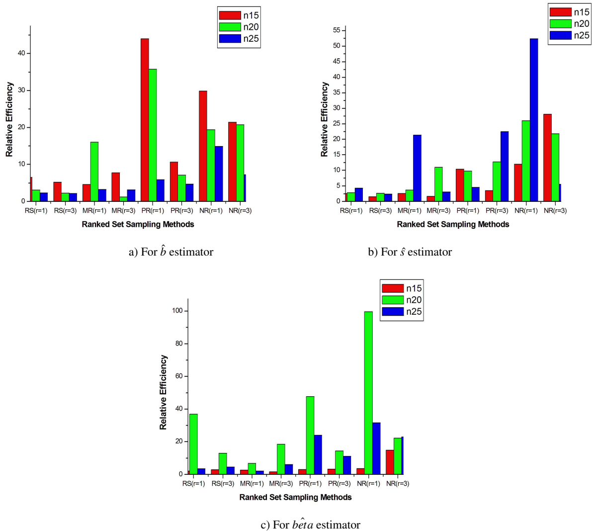
Fig. 2: Shows the REs of the estimators for G/G(3, 3, 3) .
