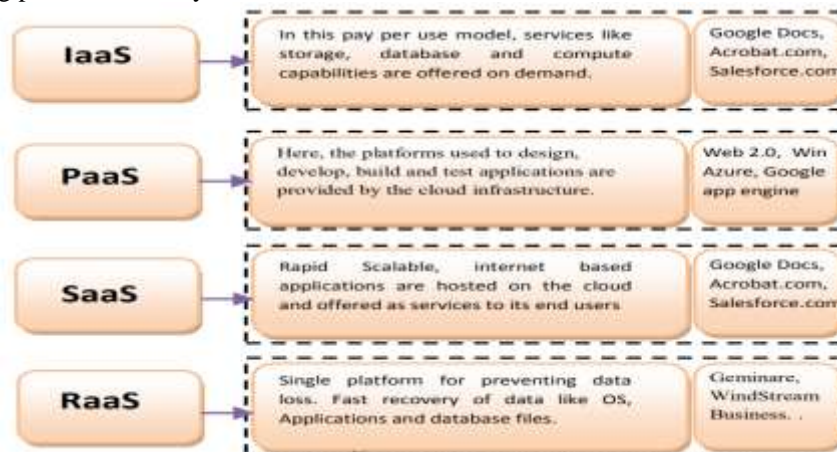
Fig.2: Cloud services [13].
