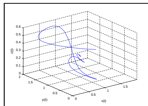
Fig. 6: Phase portrait of the system (3) for \alpha = 1.9
