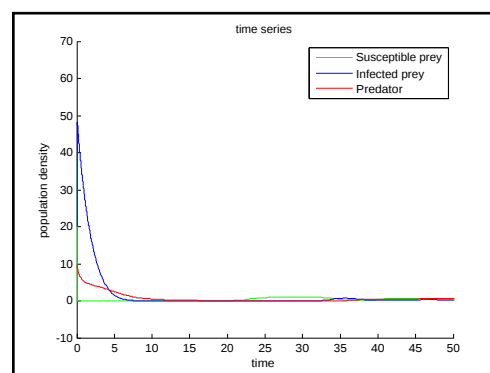
Fig. 7: Time series of the system (16) approaches asymptotically to (0,0,0) for \alpha = 1.9
