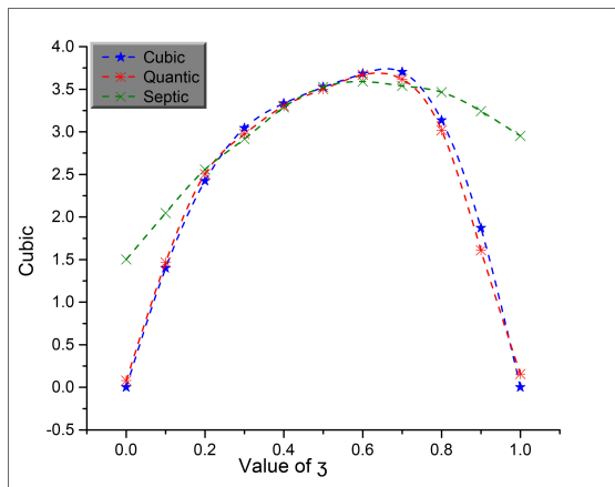
Fig. 8: The obtained absolute value of error via cubic, quantic, and septic spline schemes
