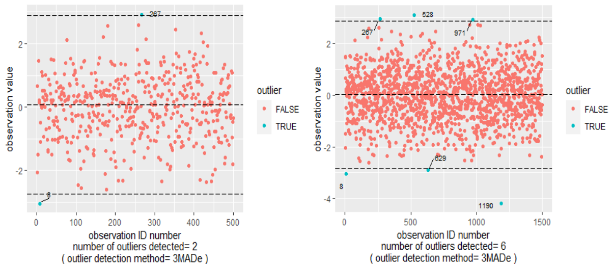
Fig. 7: Outlier detection output for 3 Median absolute deviation rule method.
