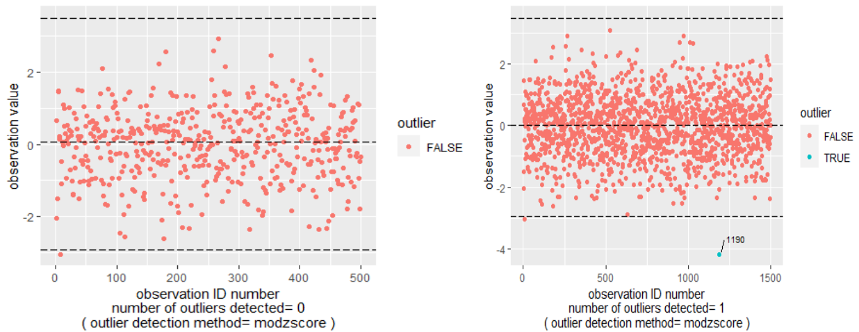
Fig. 4: Outlier detection output for modified z-score method.
