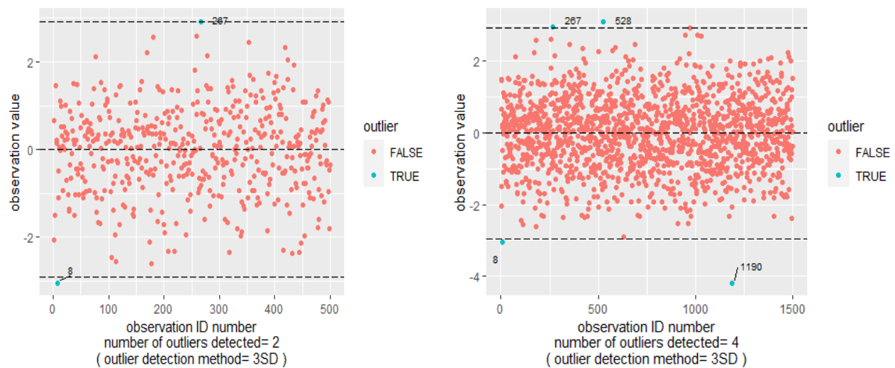
Fig.2: Outlier detection output for Three Standard deviation method.
