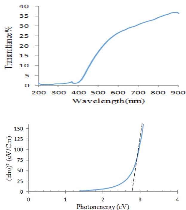
Fig.3: Transmittance Spectra of CdO thin film and (\alpha h\nu)^2 versus photon energy gap of CdO thin film continuously.
