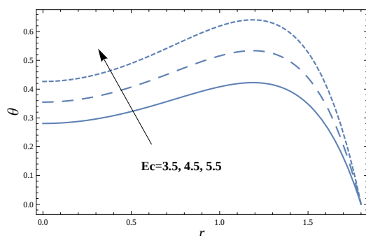
Fig. 3: the temperature profiles are plotted versus r for different values of Ec for a system have the particulars M = 1, D_a = 0.9, Gr = 0.1, Br = 0.1, h = 1.8, \frac{\partial p}{\partial z} = 1.5, Pr = 2.5, Nt = 3.5, Nb = 1.5, \lambda_1 = 0.01 and Q_0 = 1
