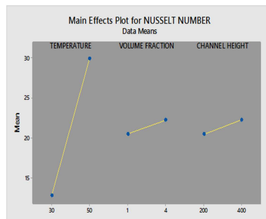
(a) Main effects plot for Nusselt number
