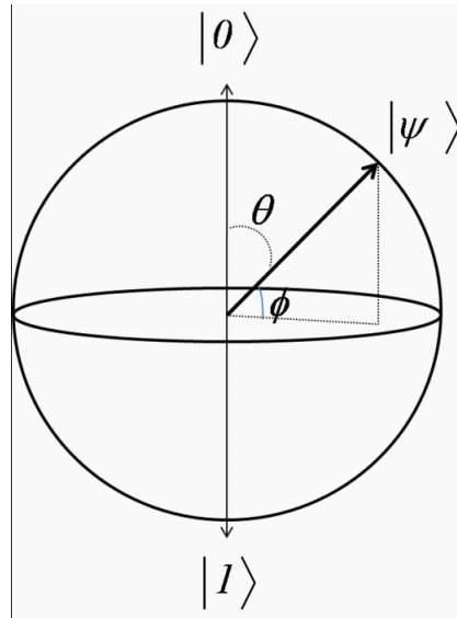
Figure 2.1: The Bloch-Poincaré sphere.
