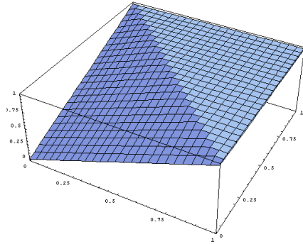
Figure 5.3: The Łukasiewicz function
