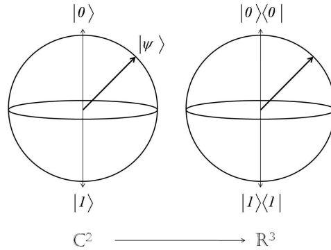
Figure 3.2: The Bloch-Poincaré sphere and the three-dimensional sphere: two different representations, in \mathbb{C}^2 and \mathbb{R}^3 respectively, of quantum information quantities.
