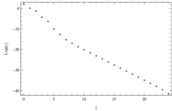
Fig. 1: Logarithmic graph of the absolute values of the coefficients, |a_j| , in the shifted Jacobi polynomial expansion for A = 10, a = 2 and \theta = \vartheta = 1 at N = 24 .
