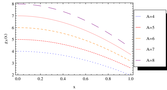
Fig. 4: Graphs of the travelling wave solution governed by (8)-(9) by the present method for A = 8, 7, 6, 5, 4 , fixed a = -5 and \theta = \vartheta = 1 at N = 8 .
