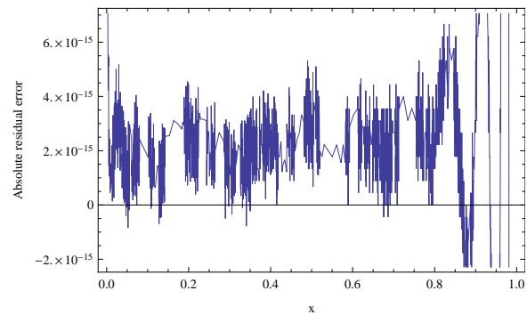
Fig. 2: Graph of absolute residual error function for A = 10, a = 2 and \theta = \vartheta = 1 at N = 24 .
