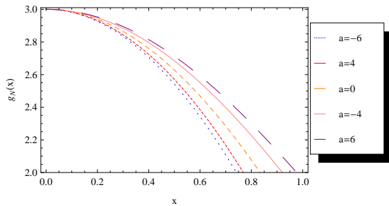
Fig. 3: Graphs of the travelling wave solution governed by (8)-(9) obtained by the present method for a = 6, 4, 0, -4, -6 , fixed A = 3 , and \theta = \vartheta = 1 at N = 8 .
