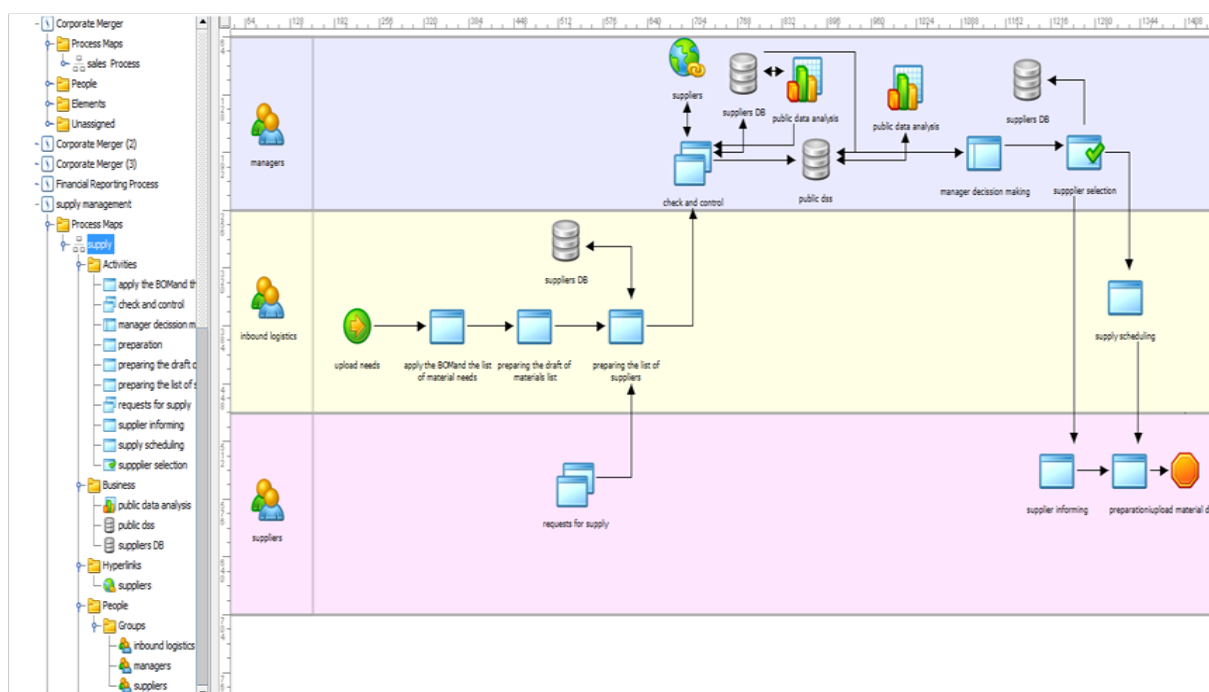
Fig. 5: A Simulation.
