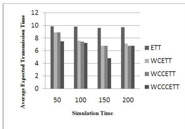
Fig. 9: Comparison of ETT, WCETT, WCCETT and WCCETT metrics in 3-channel 2-hop path.
