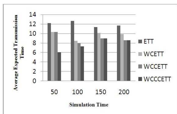
Fig. 10: Comparison of ETT, WCETT, WCCETT and WCCETT metrics in 3-channel 3-hop path.
