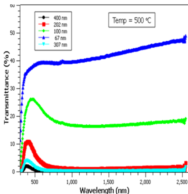
Fig. 6(b): Tungsten oxide films deposited at 500°C illustrating transmittance dependence on thickness of the films.
