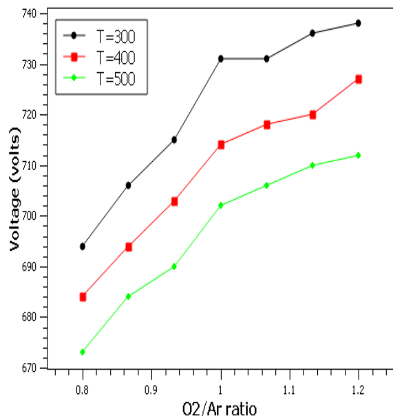
Fig. 1(b): Voltage dependence on O_2/Ar ratio.
