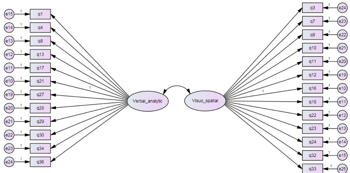
Figure 1: A hypothesized CFA model of the Visuospatial and the Verbal-analytic factors
