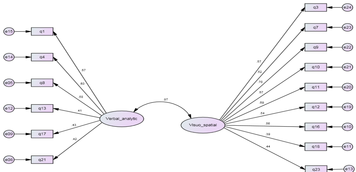
Figure 2: The final CFA model of the Visuospatial and the Verbal-analytic factors.
